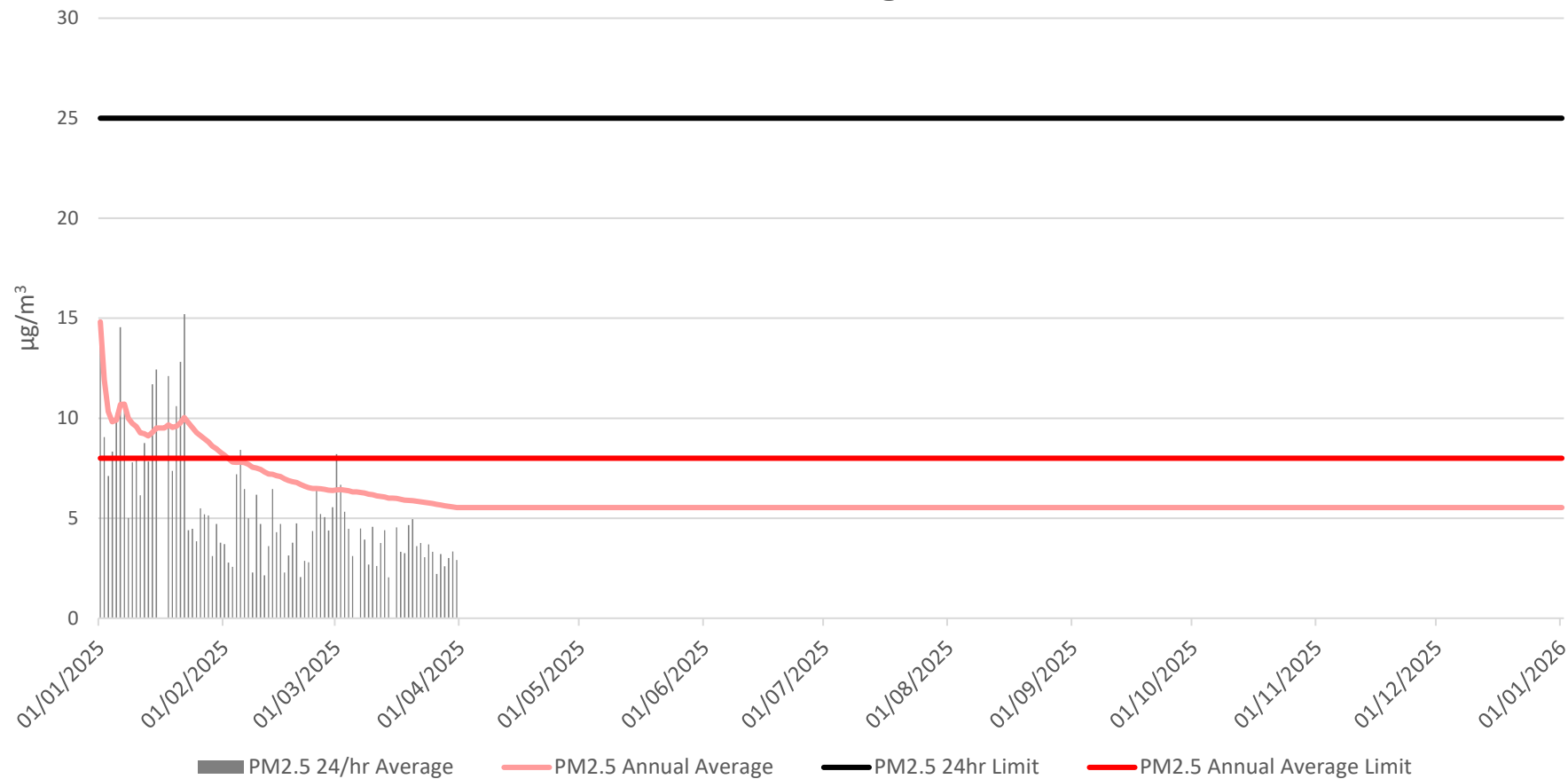
PM2.5 Monitoring - 2025
